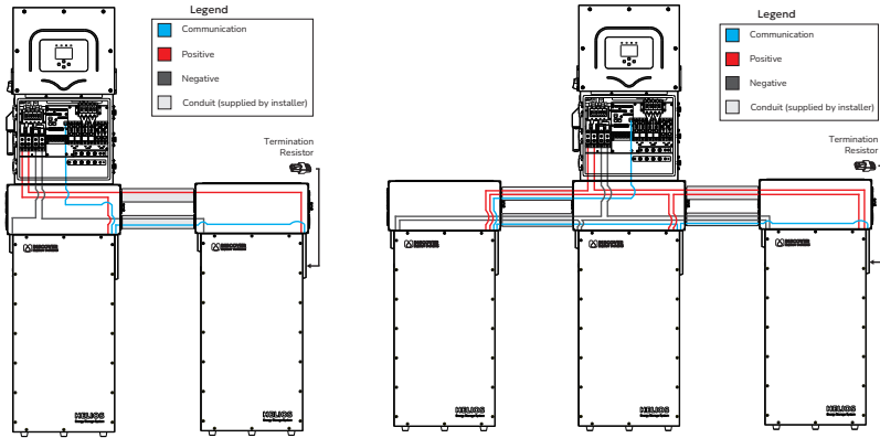
Figure 16. Direct Communication Between Inverter and Batteries
